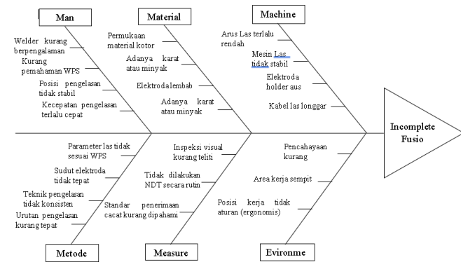
Gambar 4.4 Diagram Fishbone Incomplete Fusion
