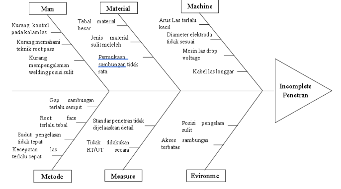
Gambar 4.7 Diagram Fishbone Porosity
